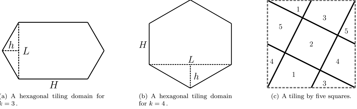
Figure 13: The case of T(1, 1) .
